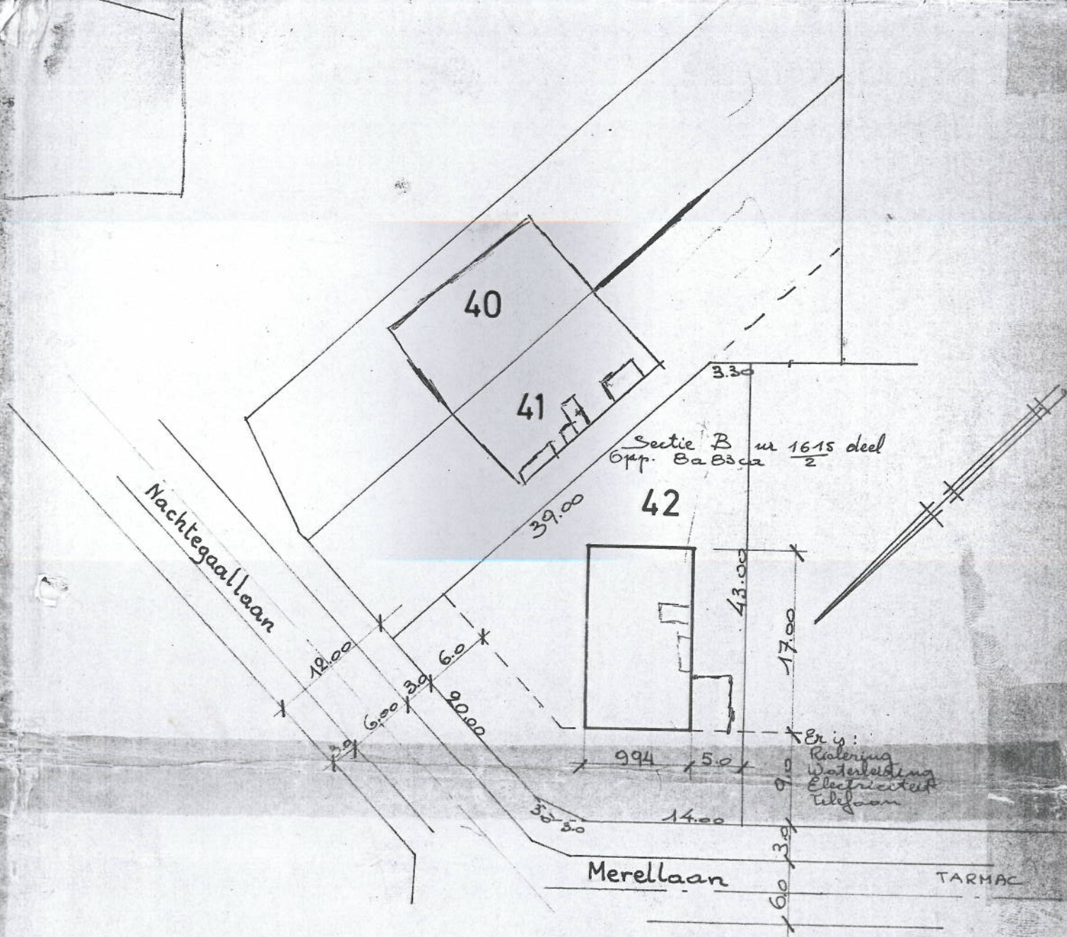
INPLANTINGSPLAN 1/500
